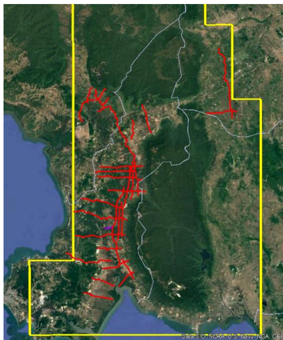
Figure 1 seismic lines depicted in red covering five basins.
